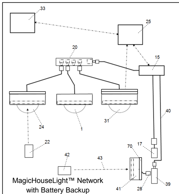
FIG. 5: MagicHouseLight™ (illustrations from the Patents)
